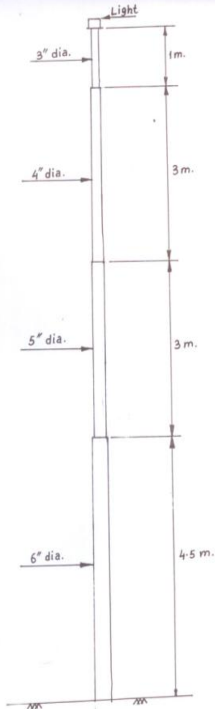
DRAWING FOR FABRICATION, PAINTING AND SUPPLY OF 11.5 m., 3mm. THICK M-S PIPE.
